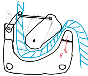
(b) Device when the pinching mechanism is actuating.
